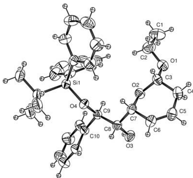
Figure 1. X-ray crystal structure of 5g .
